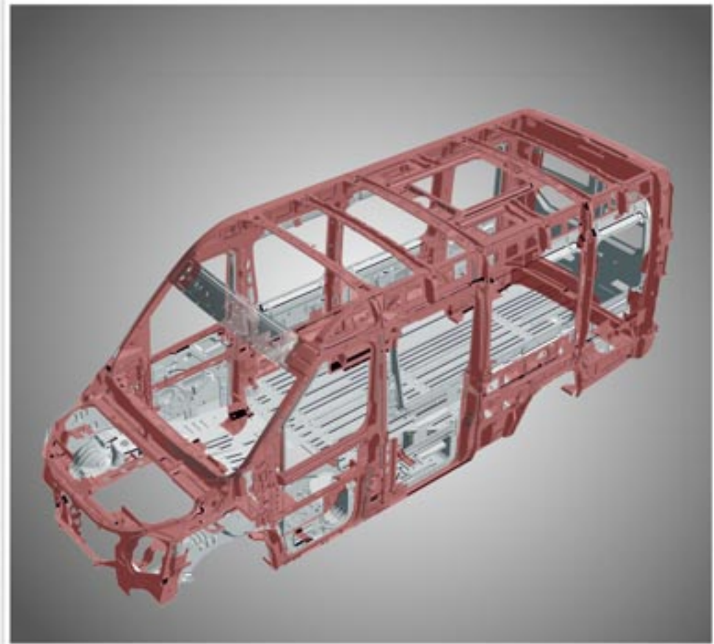
Frontal Crash Compliant Monocoque Structure
